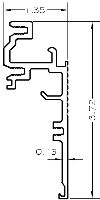
12 - HEADER LOWER BACK 6063-T5 ALLOY
