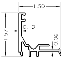
53- GLAZING BASE (311-009B)
