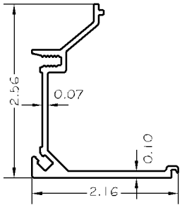
67 - LG HEADER LOWER CLOSURE FILLER 6063-T5 ALLOY
