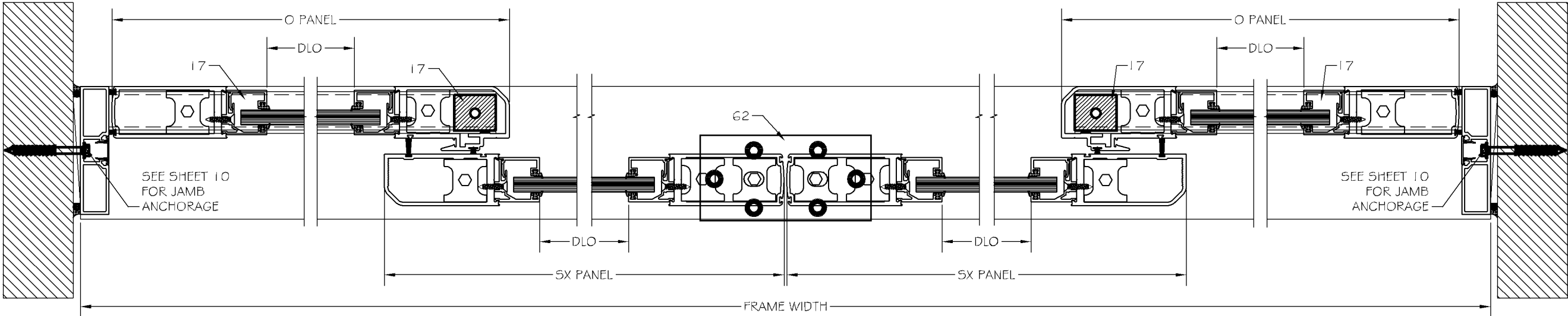
SECTION H1
