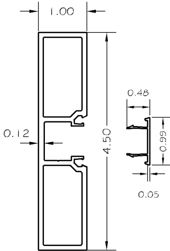
28 - JAMB WITH SNAP COVER 6063-T5 ALLOY
