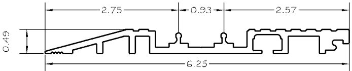
13 - FULL BREAKOUT TRACK 6063-T5 ALLOY
