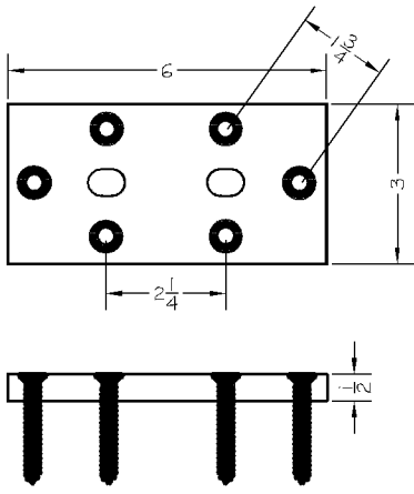
62 - FLOOR LOCK STRIKE PLATE - STEEL
