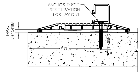
THRESHOLD SILL ANCHORAGE DETAIL INTO CONCRETE
