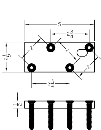
60 - FLOOR LOCK STRIKE PLATE - STEEL
