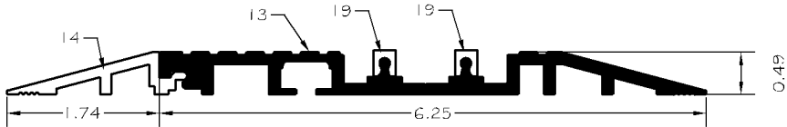
14 - THRESHOLD RAMP 6063-T5 ALLOY
